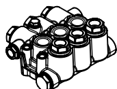
P9.040.025 TESTATA COMPLETA PISTONE ø22 POMPA GM-1 CW - COMPLETE HEAD OF THE PUMP
